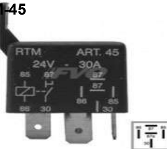
MINIRELAY 24V - 5TERM C/SOP
